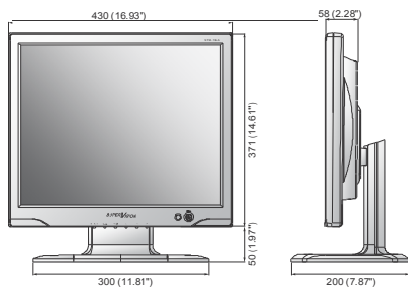
STM-19LM
